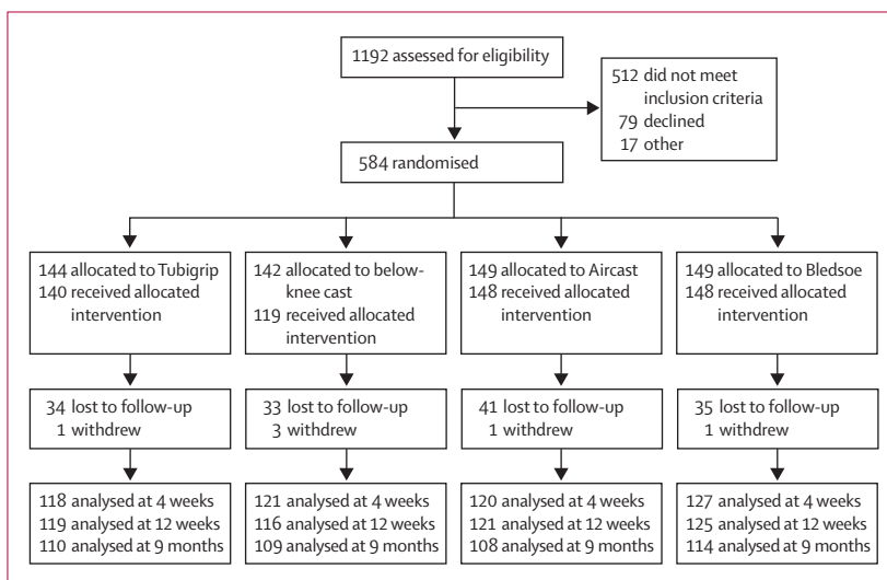
Figure 1: Trial profile
